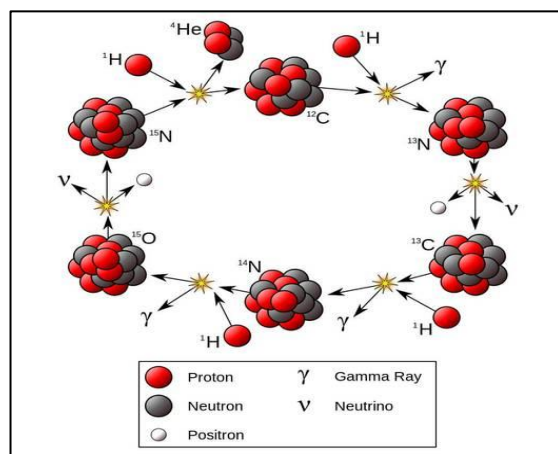
Figure 7 The CNO Cycle
