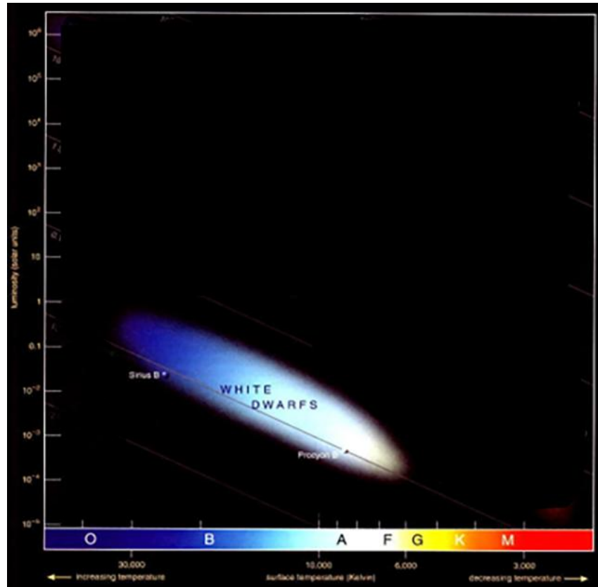
Figure 9 White Dwarf Branch on the H-R Diagram
