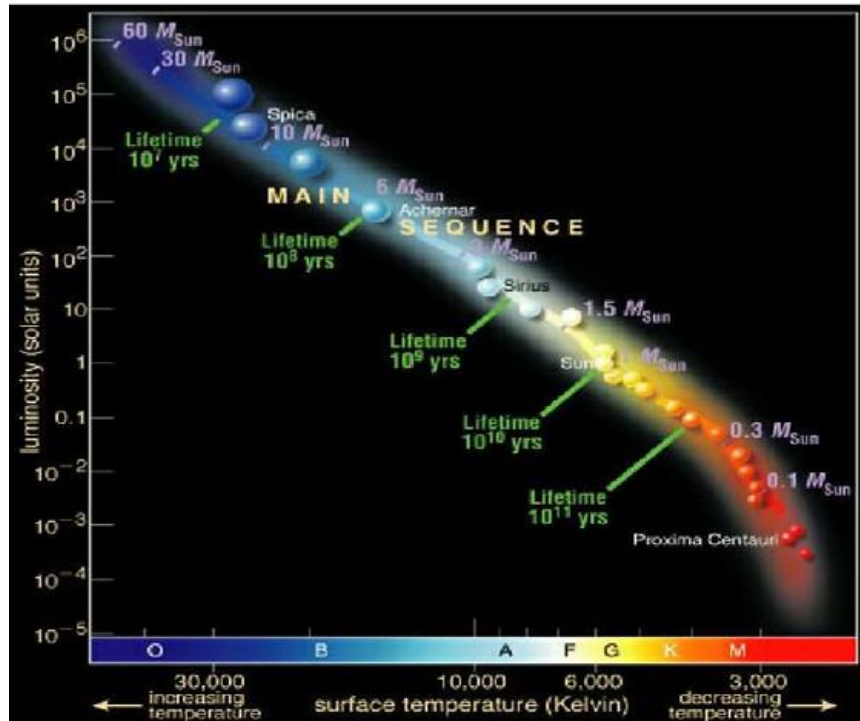
Figure 5 The Main Sequence
