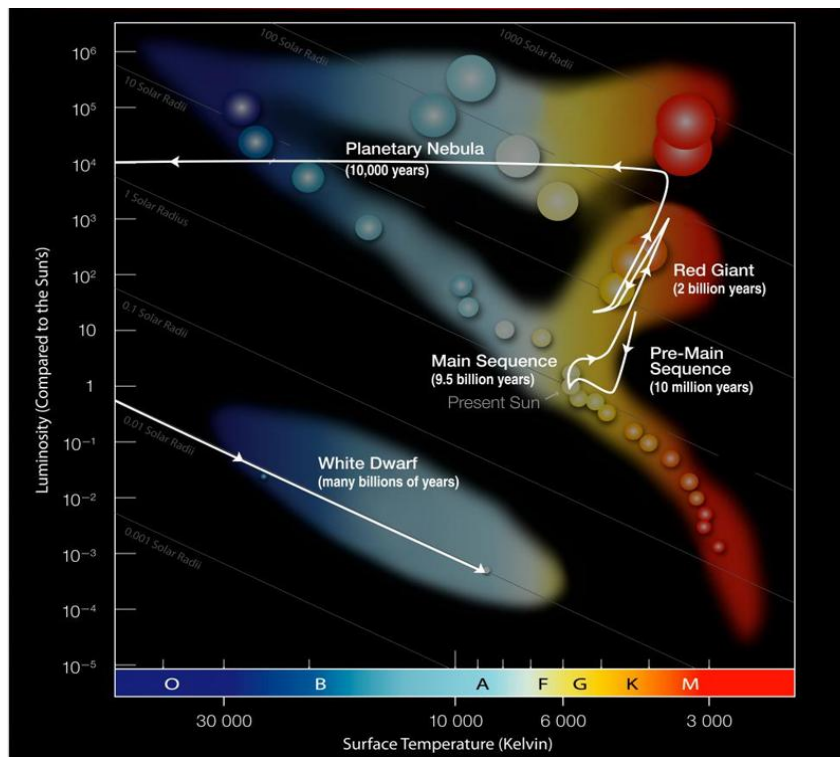
Figure 12 Evolutionary Track of the Sun
