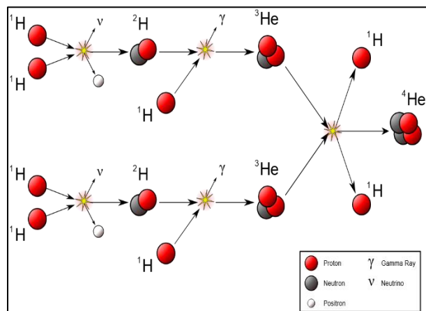
Figure 6 The Proton-Proton Chain
