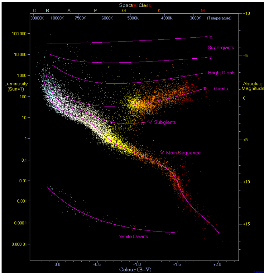
Figure 3 The Hertzsprung-Russell Diagram – Approximately 2500 real stars plotted
