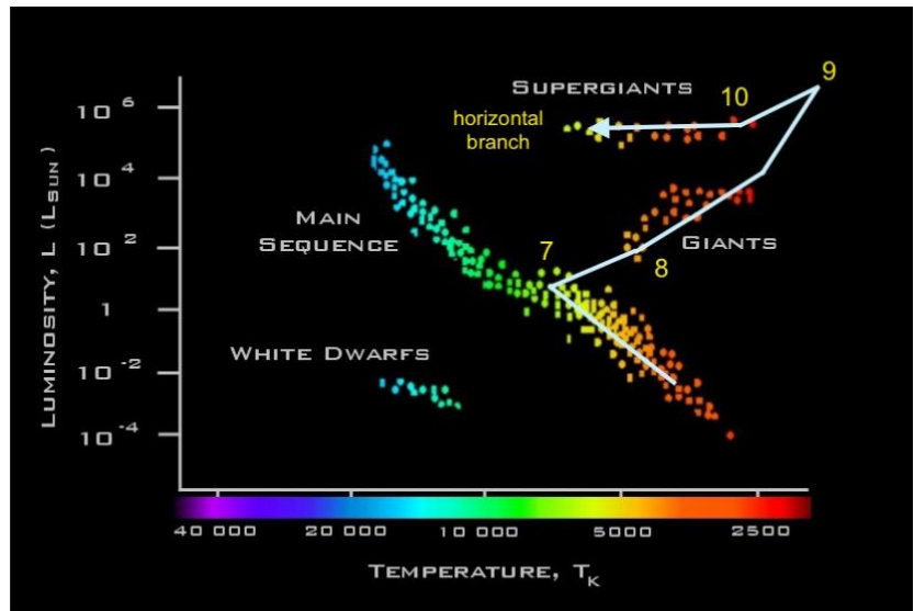
Figure 11 The Horizontal Branch
