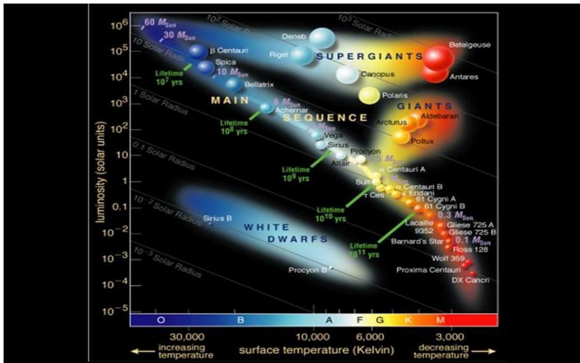
Figure 4 The Hertzsprung-Russell Diagram
