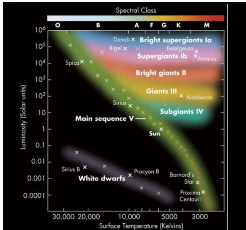
Figure 10 The subgiant and giant branches.
