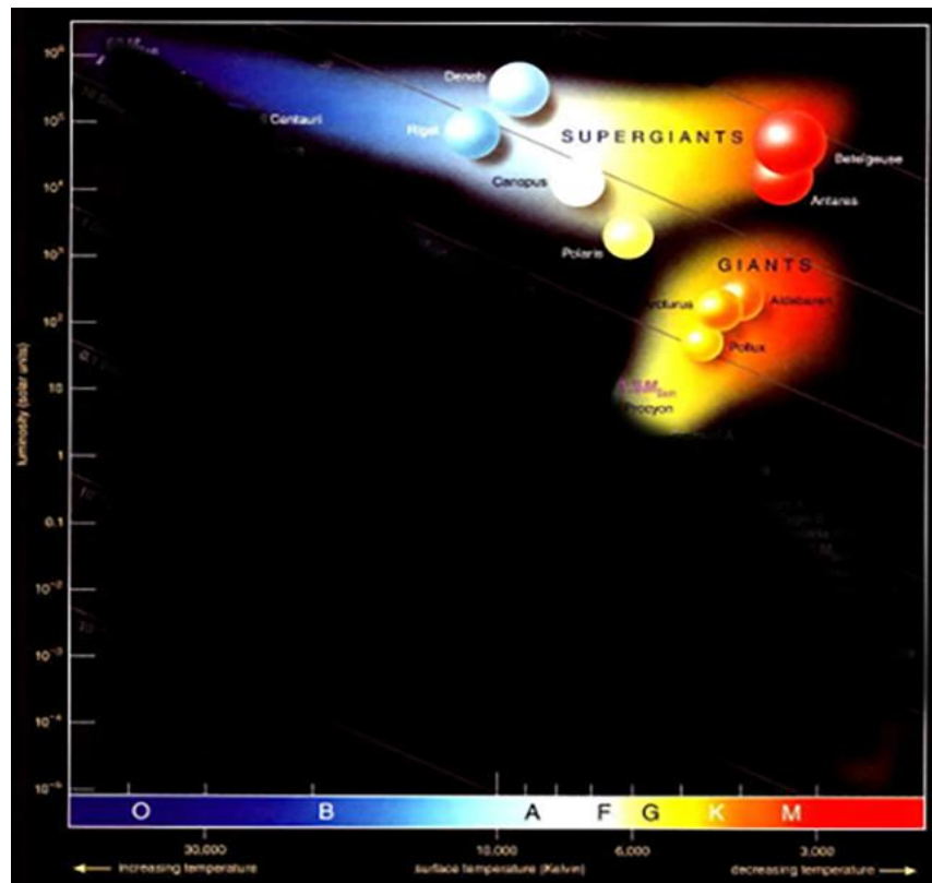
Figure 8 Giant and Supergiant Branch on the H-R Diagram
