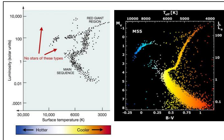
Figure 14 Left: Schematic HR diagram of a globular cluster. Right: Color Magnitude (HR) Diagram of M55 from real data
