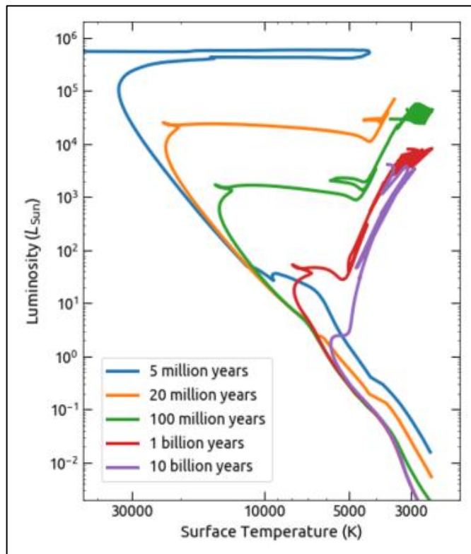
Figure 13 Theoretical isochrones for a range of ages.
