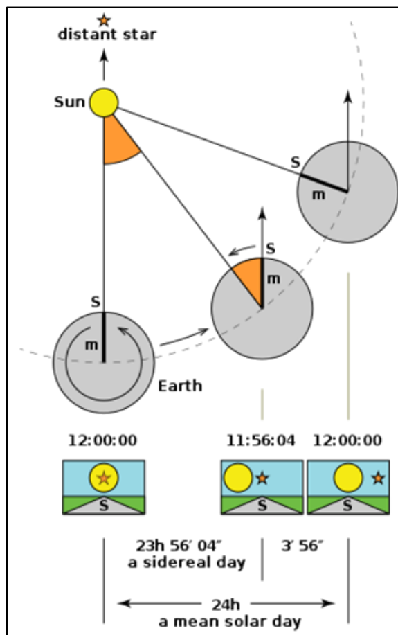
Figure 8: Solar and Sidereal Day
