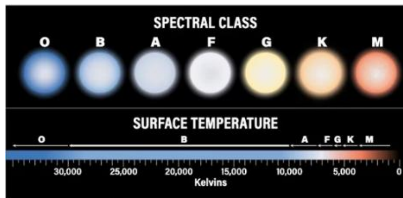
Figure 9 Spectral Classes
